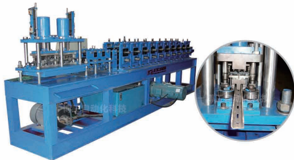
C/Z快速换型檩条机 C/Z Purlin Automatic Changeable Forming Machine
